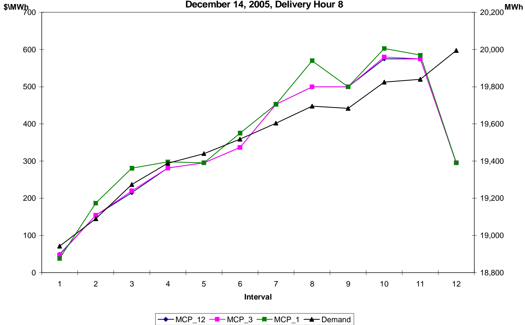
Large Contingency with No Spare Fossil Generation On Line Loss of 216 MW of Imports and 480 MW Derating of Gas-Unit December 14, 2005, Delivery Hour 8
