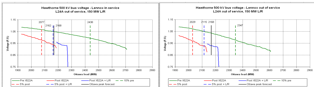
Figure 18: Hawthorne 500 kV P-V curve - L24A out of service, 150 MW L/R
