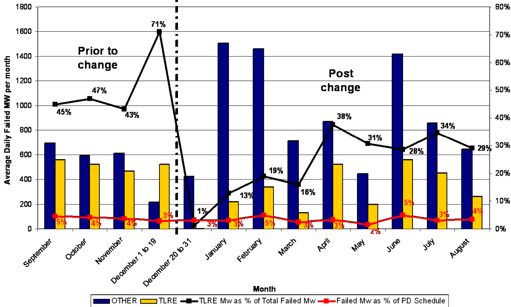
Failed MW between Ontario and New York (from September 1, 2007 to August 31, 2008)
